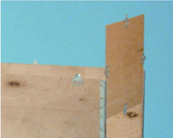
5. Pull the sides apart so the tongues can slide into the slots. Seal the tongues.
